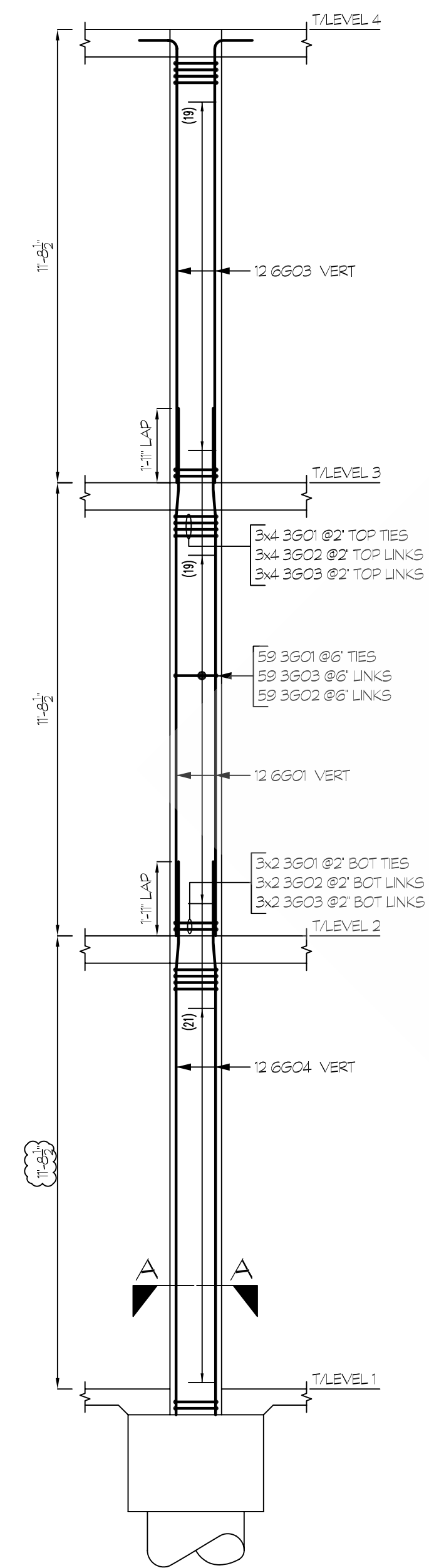
COLUMN - C1h SCALE: 1/32"=0' SDR: 65402 (1 LOC)
