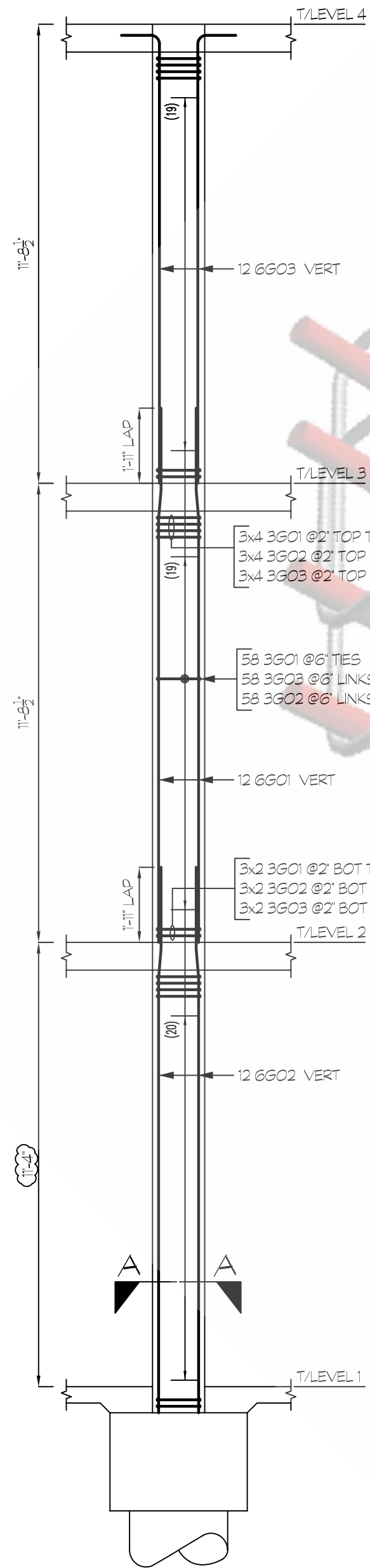
COLUMN - C1j SCALE: 1/32"=0' SDR: 65402 (1 LOC)
